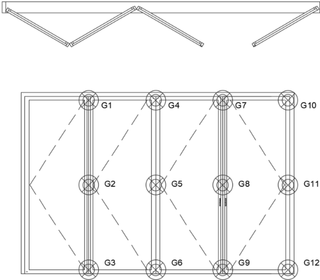
FIGURE 1: Folding Door Gauge Layout
